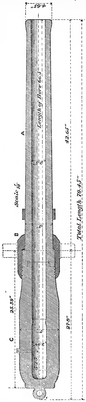
2.5 inch 7 Pr. Jointed Gun.
